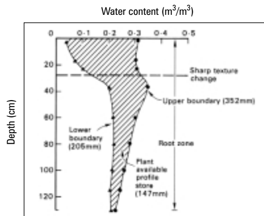
FIGURE A4.1. An example of a typical soil soil water profile determined by the NMM technique (after Williams et al. 1981)
