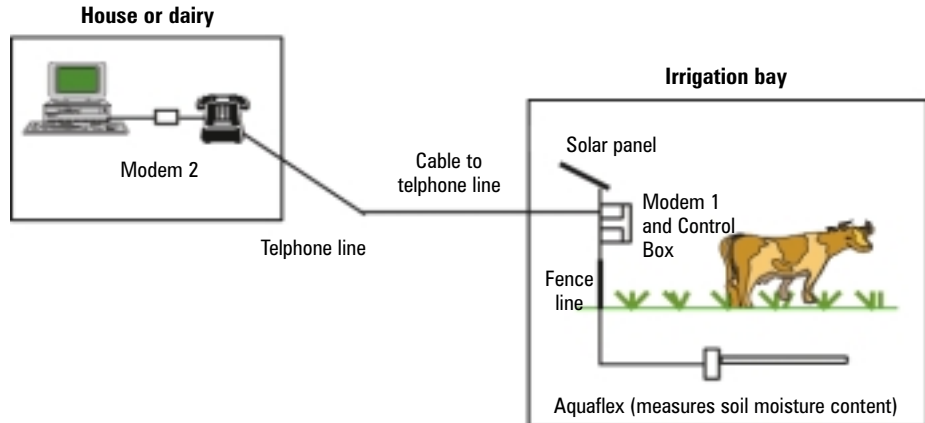
FIGURE 7.13 A schematic diagram of the irrigationscheduling system.
