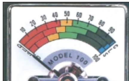
FIGURE 6.13 Aquaterr instrument and analog SWC scale.
