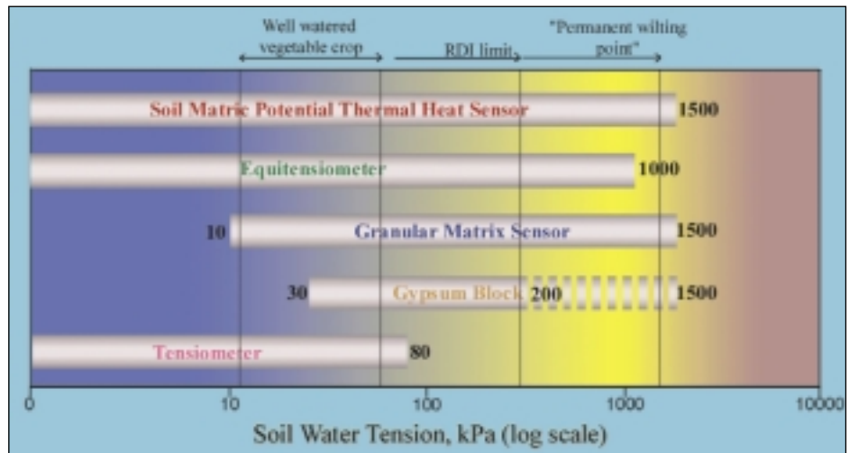
FIGURE 3.1 Measurement ranges for several soil-water-tension monitoring instruments.
