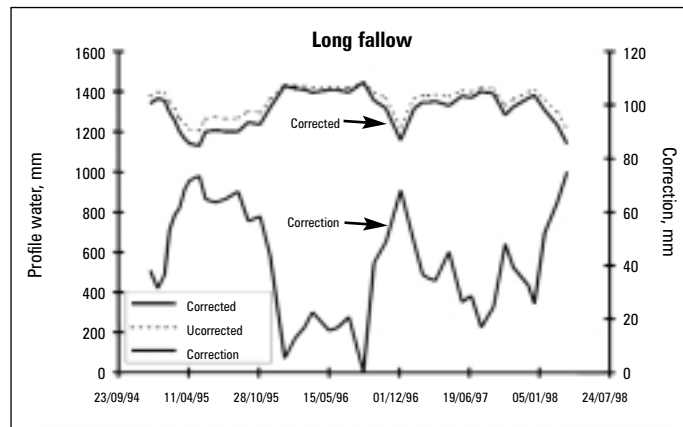
FIGURE 7.8 Estimates of profile water to 3 m depth for one treatment at 'Hudson' before and after correction, together with the actual correction.
