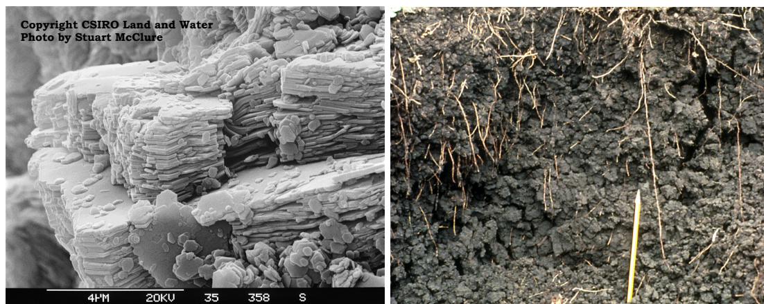
Figure 1: Soil structure at extreme scales. Left: textural porosity in the clay mineral kaolinite. The scale bar is 0.004 mm. Many of the pores visible are small enough to retain water that is not available to plants. Right: structural porosity in a “self-mulching” clay soil with well-defined aggregates and large pores that play a role in drainage, aeration, root growth and the activities of soil fauna.
