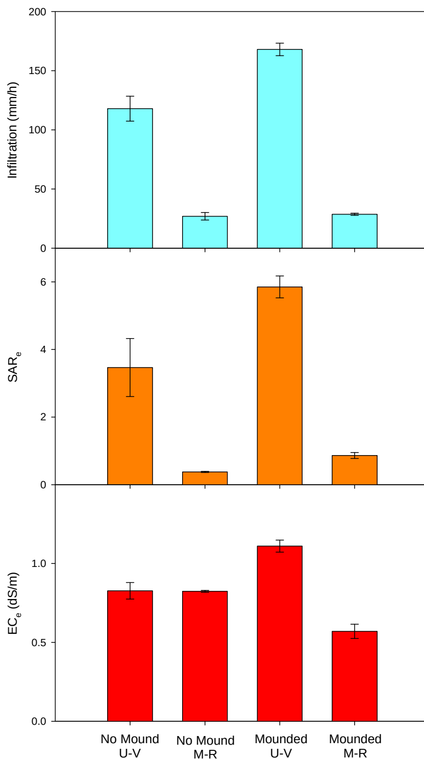
Figure 5. The infiltration rates of degassed rainwater into soil located under vine (VL) and in the mid-row (MR) in vineyards where the no soil mounding had occurred and where soil had been mounded under the vine and the EC e and SAR e in the 0-10 cm depth soil sample.
