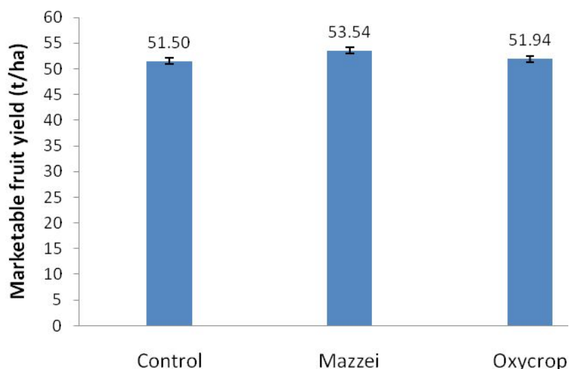
Figure 14. Marketable fruit yield (mean \pm SE) of capsicum for two different methods of oxygation in a loamy sandy soil at Bundaberg, 2009.
