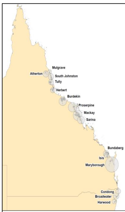
(a) Sugarcane regions in 2017
