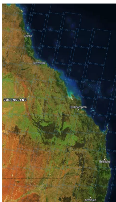
Landsat 8 data coverage
