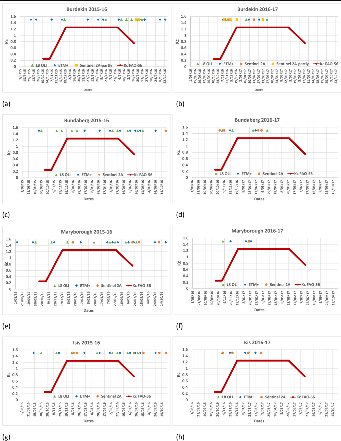
Figure 2 Temporal evolution of sugarcane crop coefficient ( K_c ) based on FAO-56 and corresponding satellite overpasses for Landsat OLI, ETM+ and Sentinel-2A during 2015-16 and 2016-17 (till March 2017) growing season (Nov-Oct) in Burdekin, Bundaberg, Maryborough and Isis regions.
