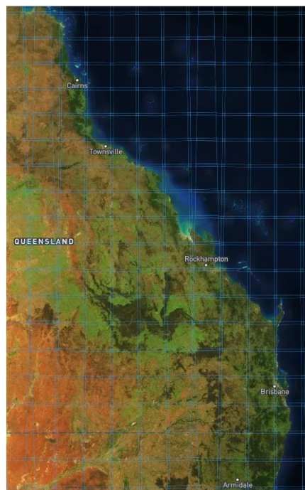
Sentinel 2 data coverage
