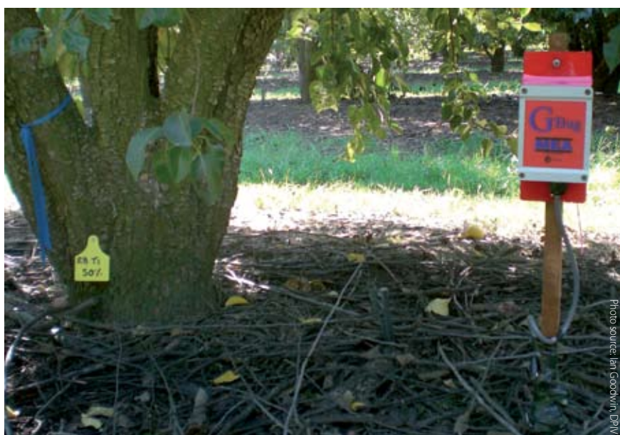
Gypsum blocks measure soil water suction.
