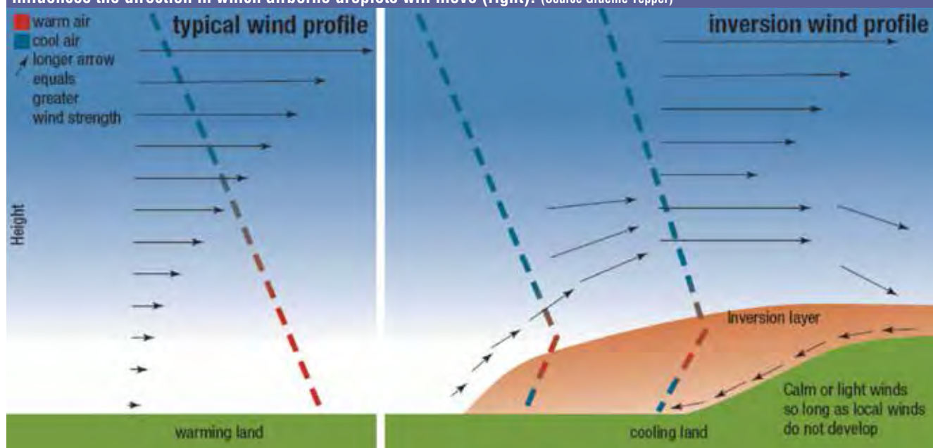
FIGURE 3: Air movement under a surface temperature inversion differs from a typical wind profile (left). Surface winds de-couple from the surface, accelerate and flow over the inversion. Within the inversion, winds are typically light and often drain down slope, regardless of the overlying wind direction. Under an inversion the shape of the landscape also influences the direction in which airborne droplets will move (right). (Source Graeme Tepper)
