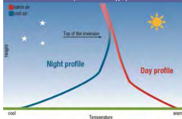
FIGURE 2: Typical vertical temperature profiles for a point in time during the night and day. At low levels, the day profile typically cools with height and the night profile typically warms with height. Little change occurs at elevated altitudes. (Source Graeme Tepper)
