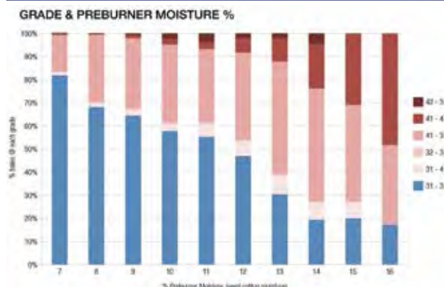
FIGURE 3: Cotton grade and pre-burner moisture percentage. (Cotton Australia)
