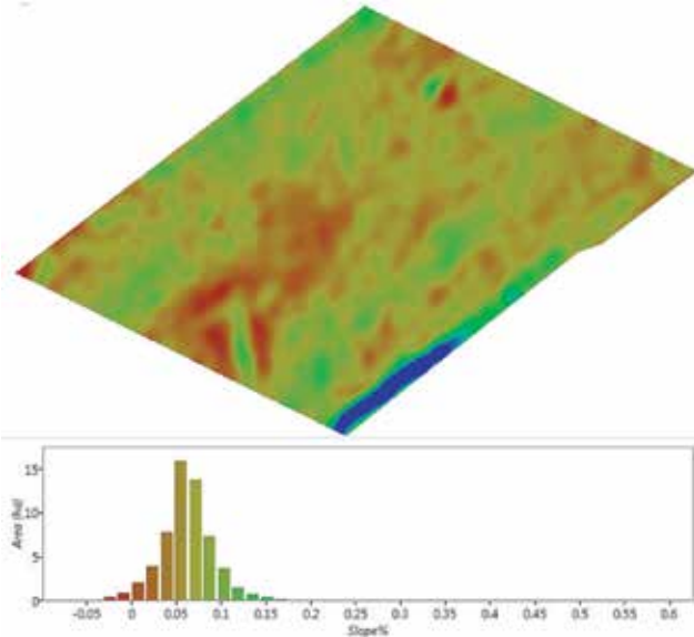
FIGURE 3: Slope% Map created from an RTK tractor steering system where the X axis shows soil level above or below a “plane of best fit (0)” as a percentage (ie. 15ha of this field is 0.05 per cent above the plane).
