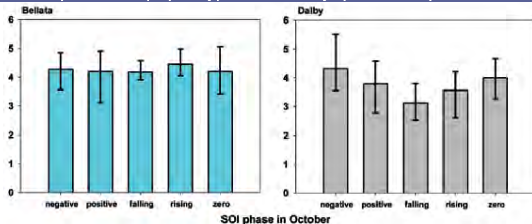
FIGURE 3: Forecasted average raingrown cotton lint yields (simulated using OZCOT using the details on the previous page for a 250mm plant available soil water profile) for single skip row configurations at Bellata (NSW) and Dalby (Qld) for different phases of the SOI in October. The bottom of the error bar is the 80 per cent probability of exceedence, while the top is the 20 per cent probability. For a 200mm plant available soil water profile, average yields are less than for a 250mm profile and there is considerably more variability estimated for the negative, positive and zero phases. Average yields are considerably less for the rapidly falling phases, but has slightly less variability.
