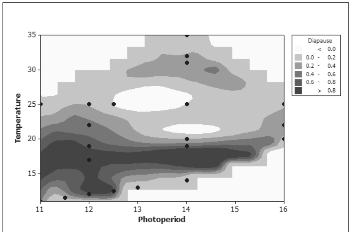
Fig. 10. Contour plot of photoperiod (hours of light/24h) temperature data (°C) for the induction of diapause (proportion) in H. punctigera .
