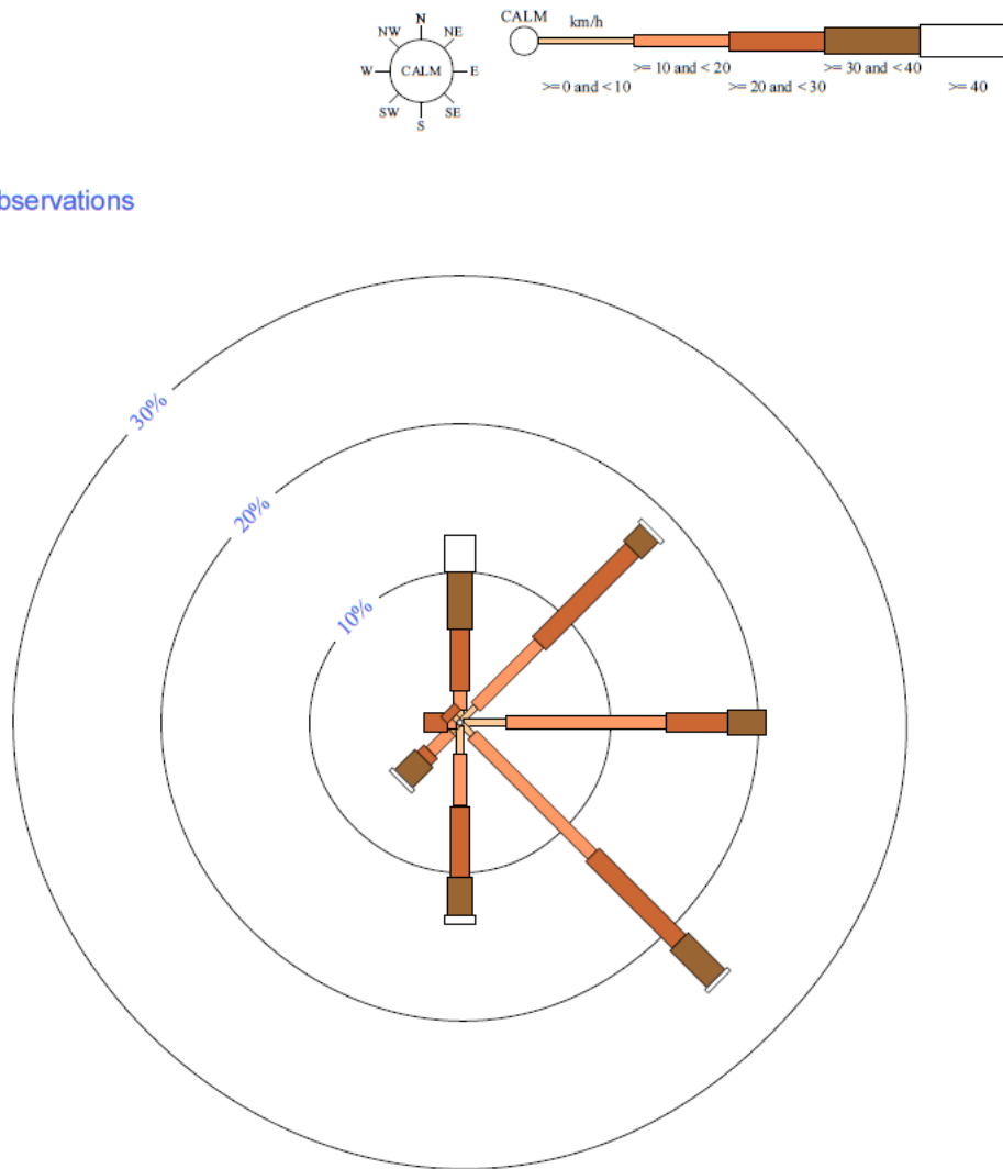
Fig. 48. Rose of wind direction versus wind speed in km/h for the month of September (averaged from 2000 to 2010) at Birdsville airport (Bureau of Meteorology).
