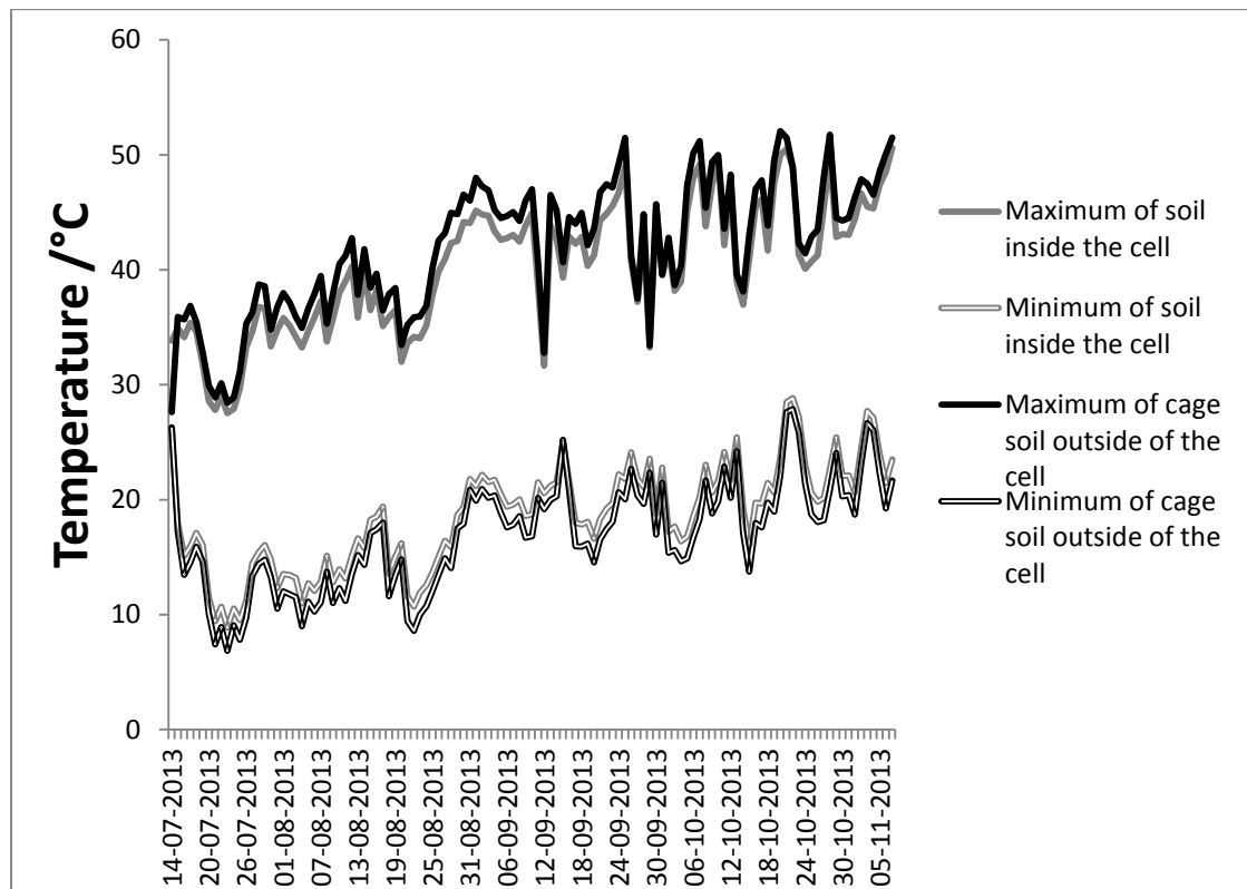
Fig. 20. Daily minimum and maximum soil temperatures inside emergence cages and inside emergence cells at "Cluny", 2013. There was a slight insulation effect of the cells, but overall there was little difference between the soil in the emergence cages, and the cells inside the emergence cages.
