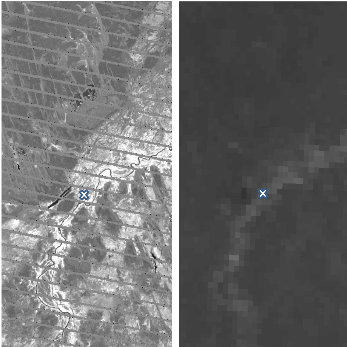
Fig. 37. Comparison of a Landsat 7 NDVI image (left) with 30m resolution (and scan-line errors) and a MODIS EVI image (right) with 250m resolution. The X denotes the same site in Birdsville (25.9S, 139.4E).
