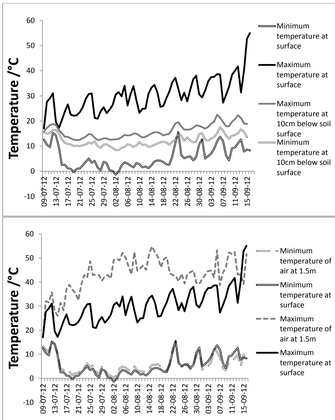
Fig 18. Daily maximum and minimum temperatures at “Monkira”, 2012. Maximum daily temperatures 1.5m in the air outside the emergence cages were higher than at the covered soil surface outside the emergence cages, but minimum daily temperatures were nearly identical at 1.5m and the soil surface (top). In contrast, both minimum and maximum temperatures recorded at 10cm below the surface inside the emergence cages showed far less fluctuations than at the soil surface outside the emergence cages (bottom).
