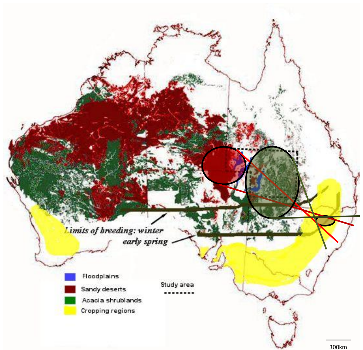
Fig. 47. Potential wind directions needed to bring inland H. punctigera from inland Queensland (red ellipse) and Acacia shrublands (green ellipse) into the Namoi Valley cropping region (brown ellipse).
