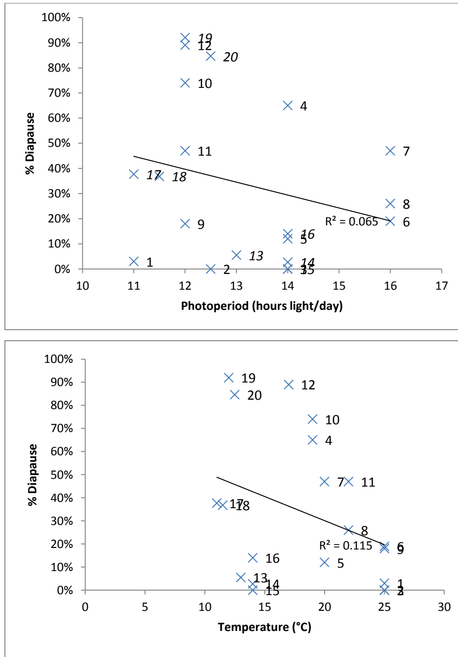
Fig. 5. Photoperiod (a) and temperature (b) and the percentage of diapause induced in H. punctigera . Numbered points represent the same experiment in each graph. Points 1-13 are from Table 3 while 14-20 are from Table 5 of Cullen and Browning (1978).
