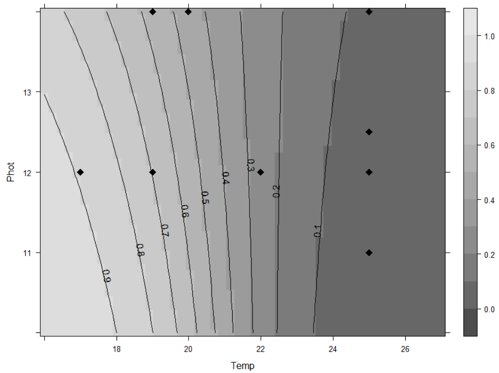
Fig. 7. Generalised linear model predictions of diapause in H. punctigera based on the data in this study. Phot= Photoperiod, Temp = temperature (°C) Study data are overlaid as diamonds.
