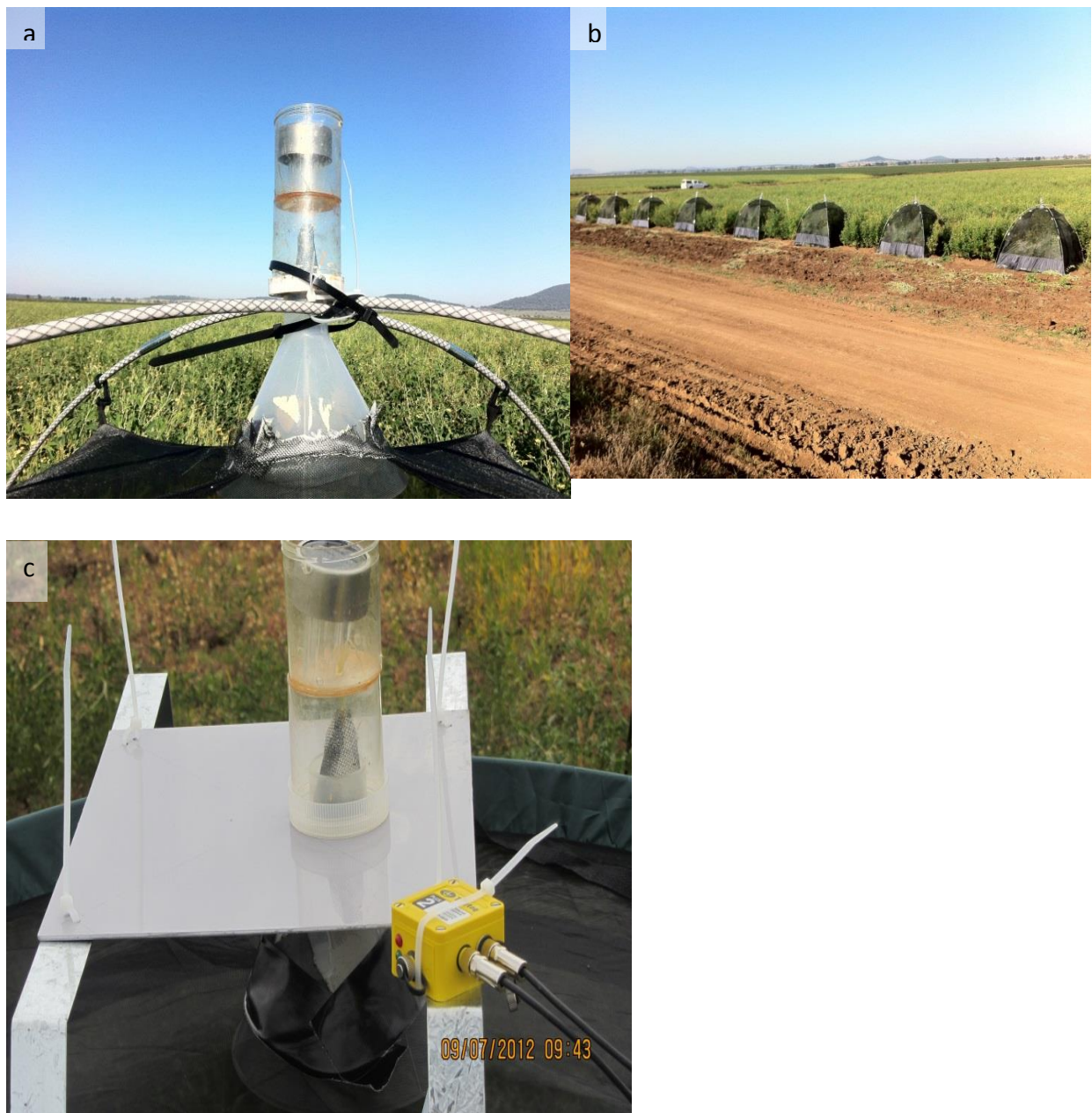
Fig. 14. Second and third iterations of emergence cage design. Fig. a) shows that the post, tensile cord and bracket were discarded in favour of strapping the capture mechanism directly to the cages, Fig. b) shows the larger cages over multiple rows, and c) shows how a custom-designed PVC sheet was strapped to the edge of the cages using aluminium brackets, to secure the catchment cup and keep it upright, even in strong winds (Photo: P. Gregg). A dual probe data logger was also attached to at least two cages.
