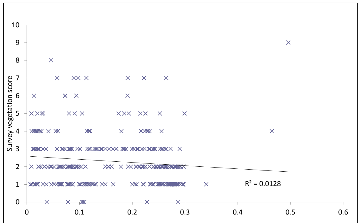
Fig. 38. Comparison between Landsat 7 NDVI and survey vegetation ratings from 2009-2012.
